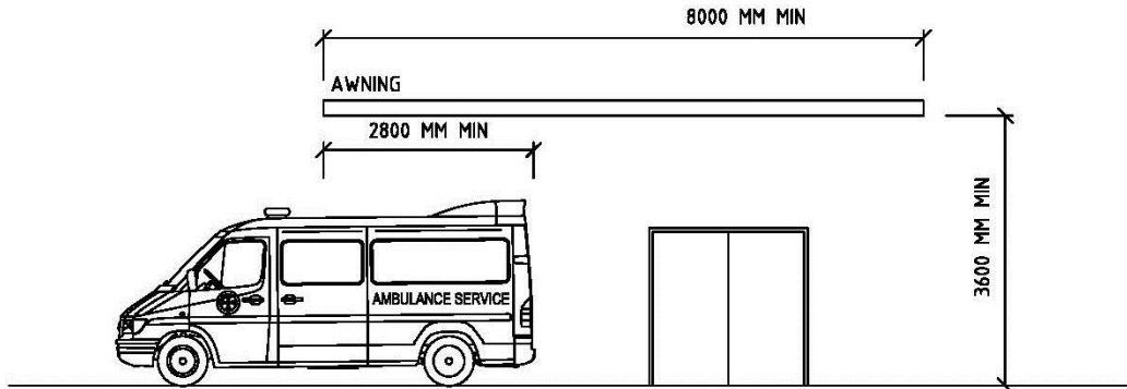
Figure 19: Ambulance Bay height clearance
