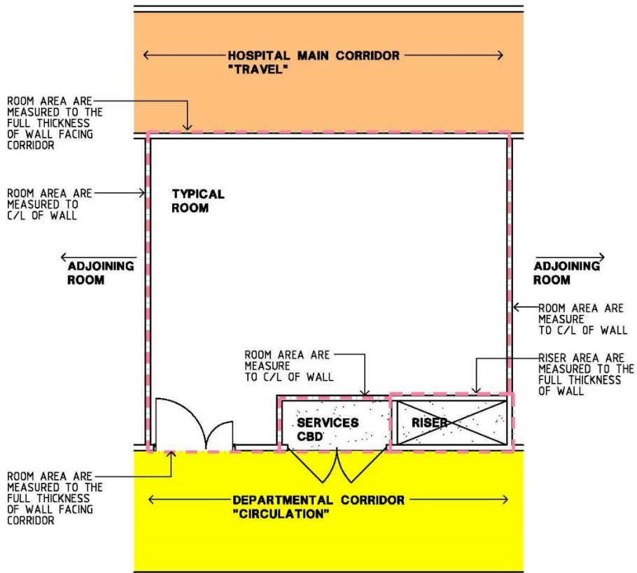
Figure 8: Typical Room between Circulation and Travel Corridors
