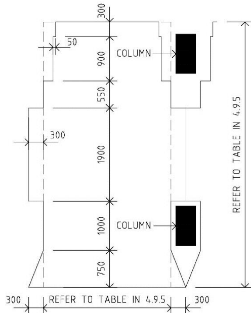
Figure 17: template for clearances within parking bay
